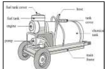
Towed wheel-mounted power sprayer Source : PNS/PAES 157:2011 p.6
