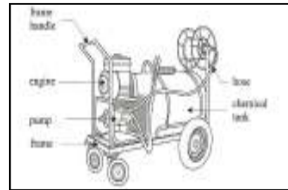
Hand-pushed wheel-mounted power sprayer Source : PNS/PAES 157:2011 p.6
